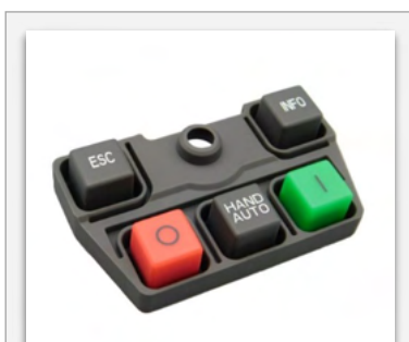
Colour insert moulding with screen printing and clear wear resistive coating
